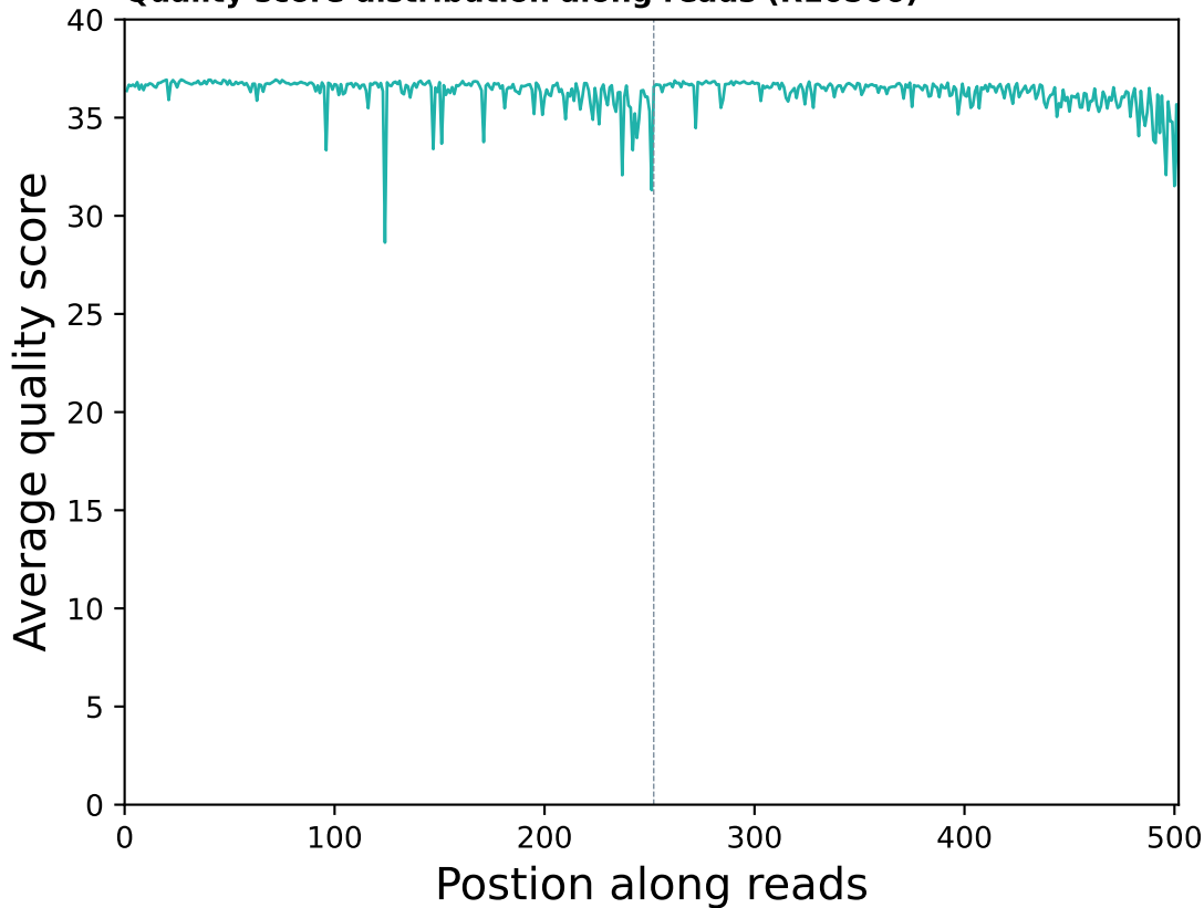
Quality score distribution along reads (R10506)
